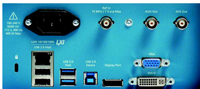
The I/O you need to connect the 6 Series MSO to the rest of your design environment.
