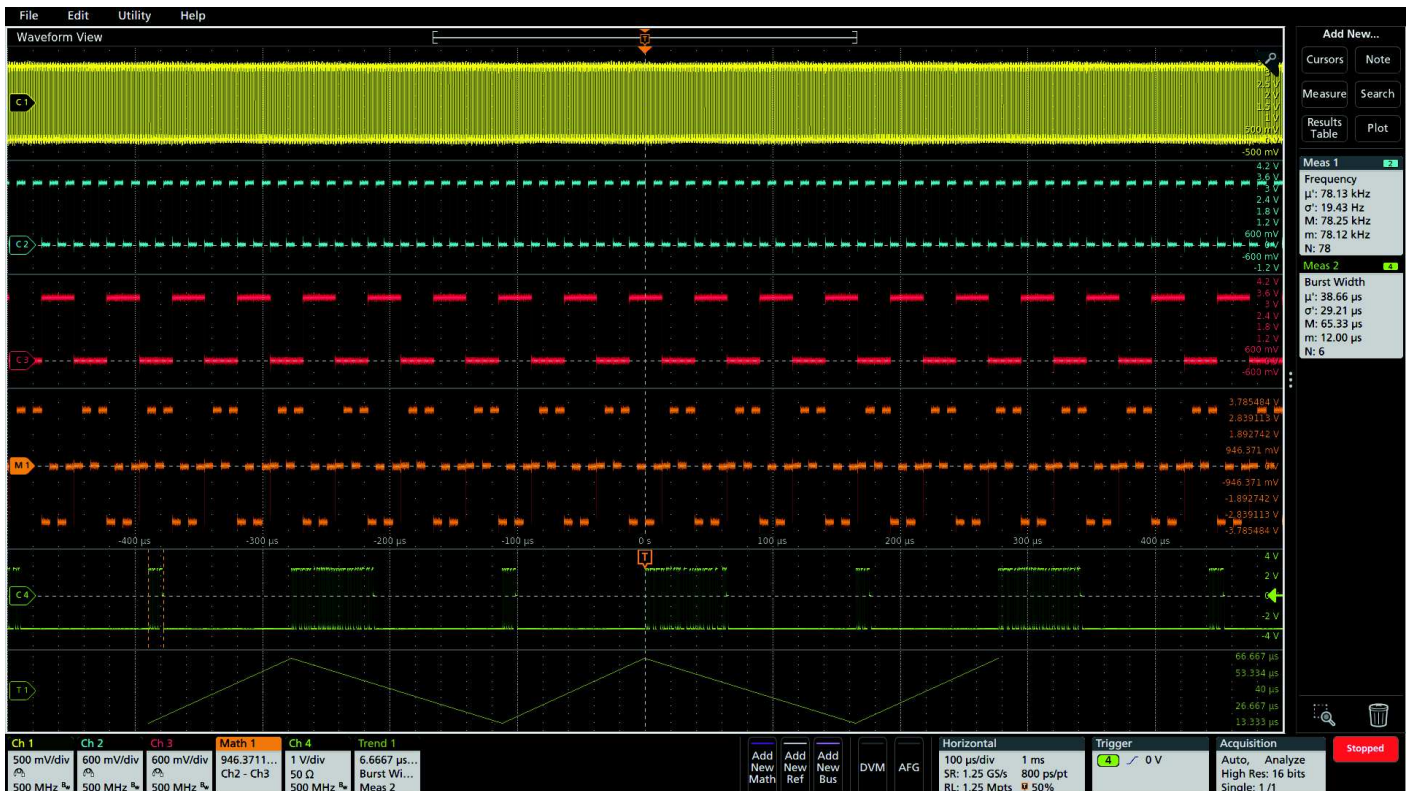
Using measurements to characterize burst width and Frequency.
